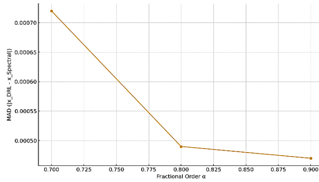
Fig. 7. Mean absolute deviation vs fractional order \alpha .
